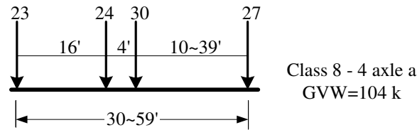
Fig. F.13 Representative vehicle for Class 8 vehicles (Type 3S1)
