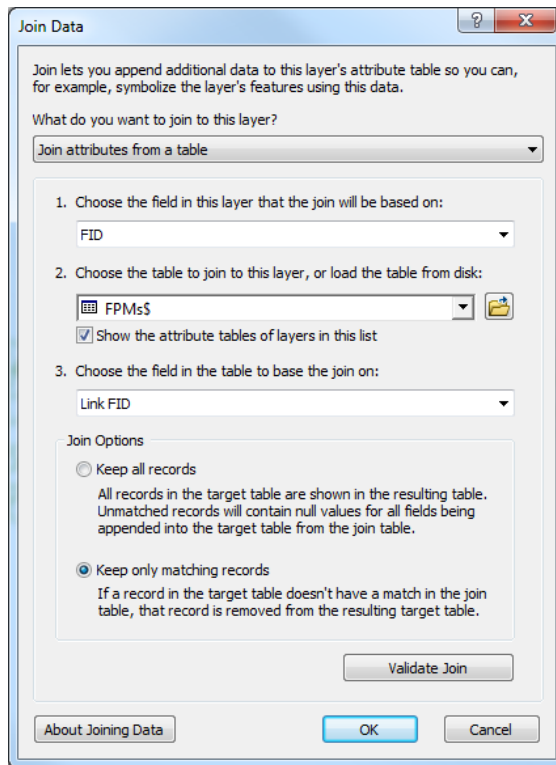
FIGURE 47 Associating FPMs with Links
