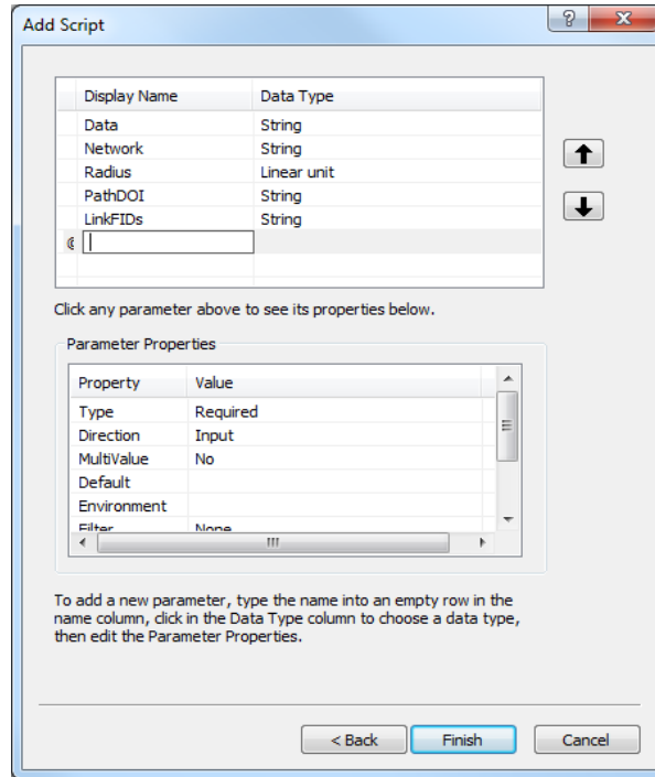
FIGURE 40 Adding New Script Window (3)
