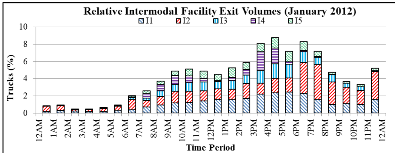
FIGURE D-3 Relative Daily Intermodal Facility Exit Volumes
