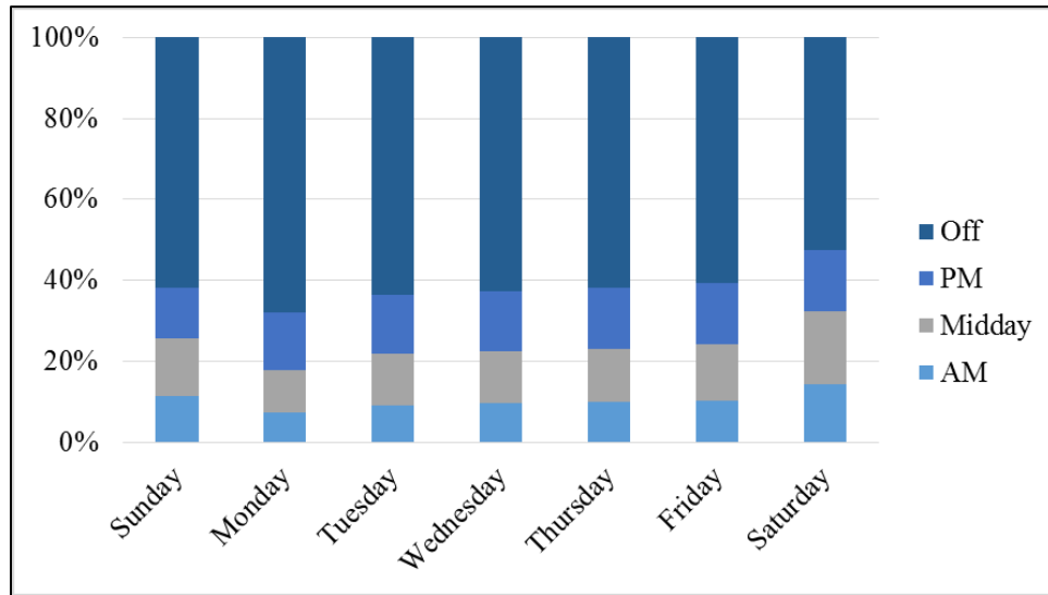
FIGURE 4 Truck Distribution by Day of the Week and Time of the Day
