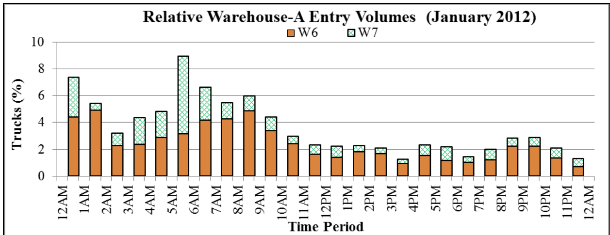
FIGURE D-9 Relative Daily Warehouse-A Entry Volumes
