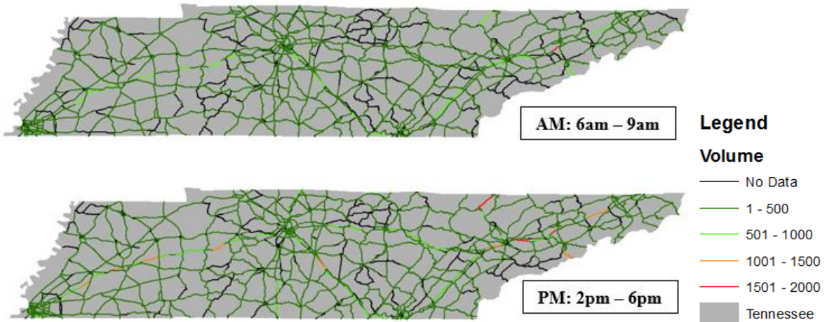
FIGURE B-15 Total Volumes, September 18 th – 20 th , AM & PM Periods
