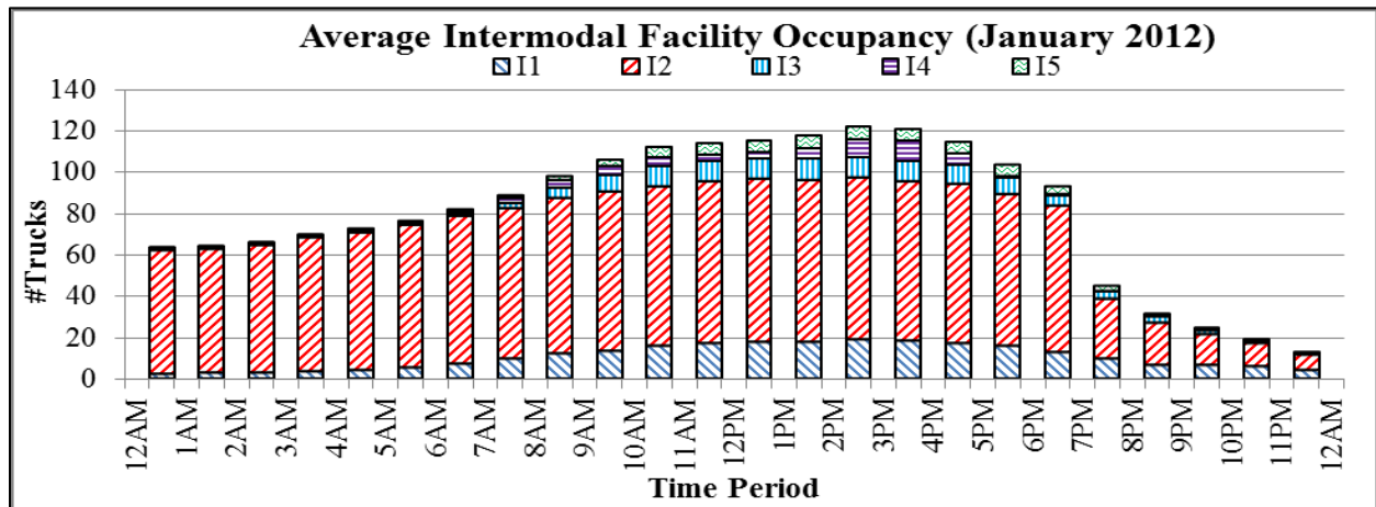
FIGURE 20 Daily Intermodal Facility Occupancy
