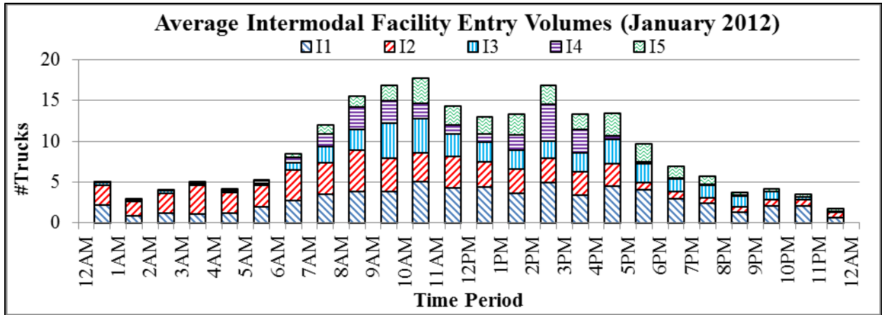
FIGURE 24 Daily Intermodal Facility Entry Volumes
