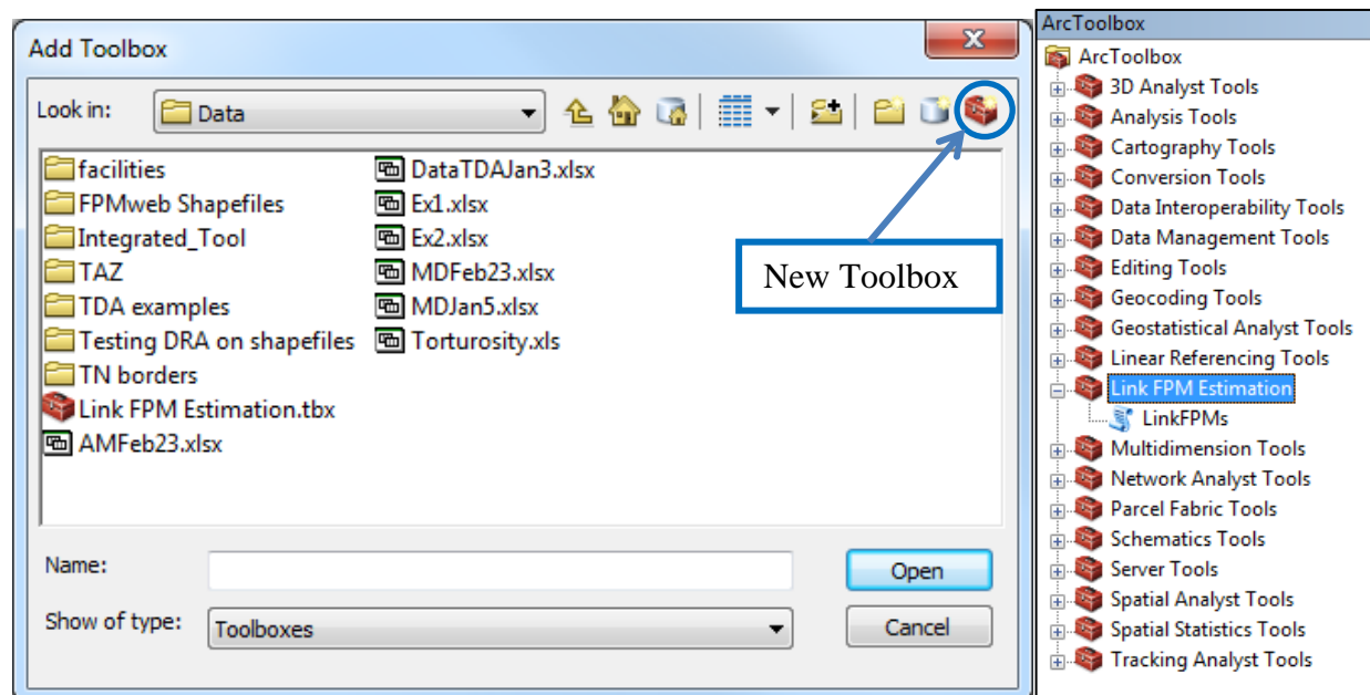
FIGURE 38 Adding New ArcGIS Toolbox
