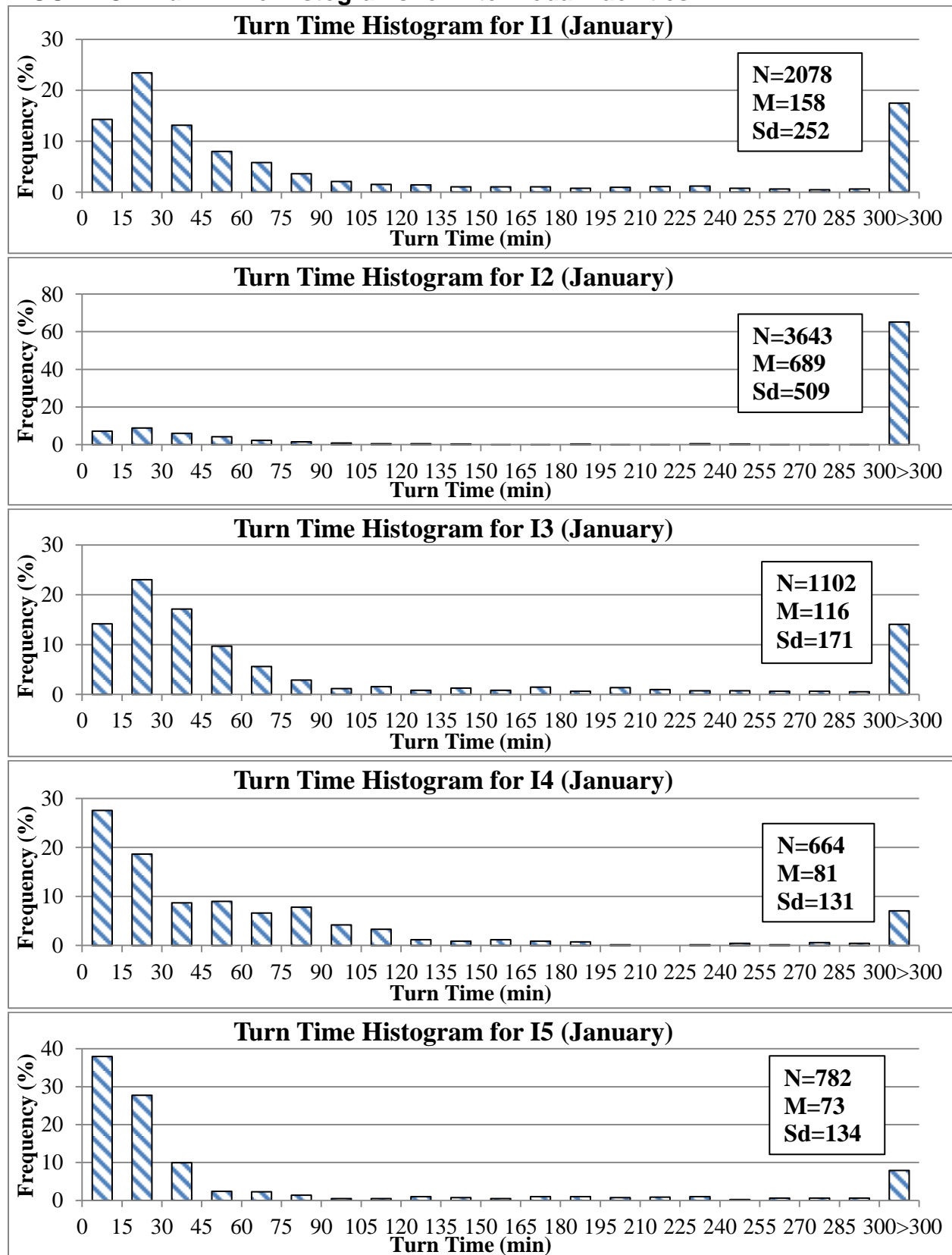
FIGURE C-1 Turn Time Histograms for Intermodal Facilities
