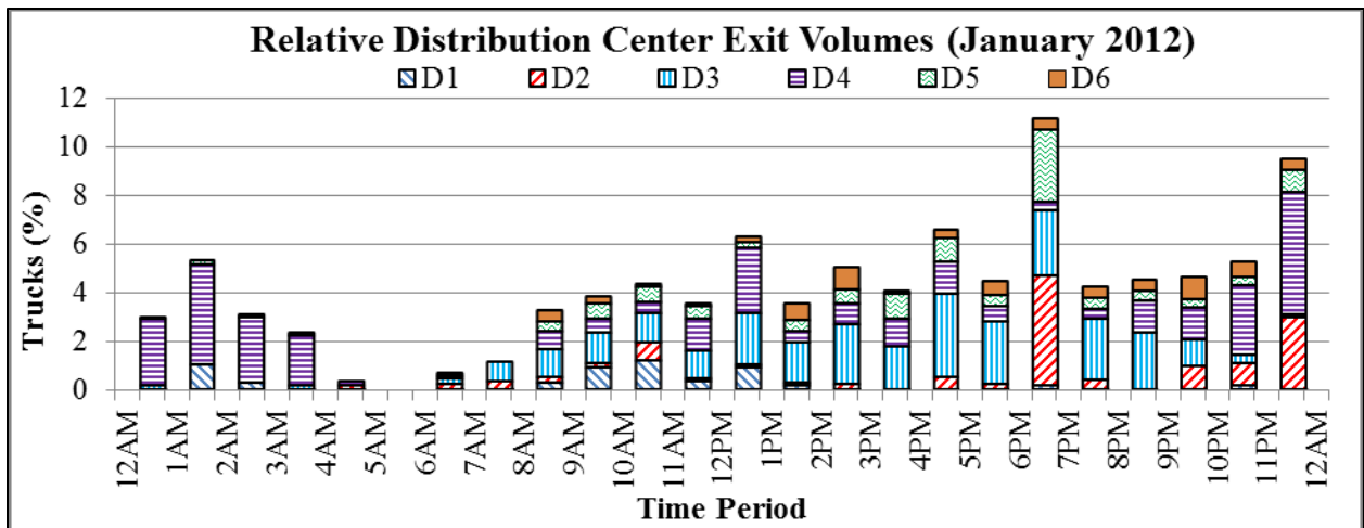
FIGURE D-6 Relative Daily Distribution Center Exit Volumes
