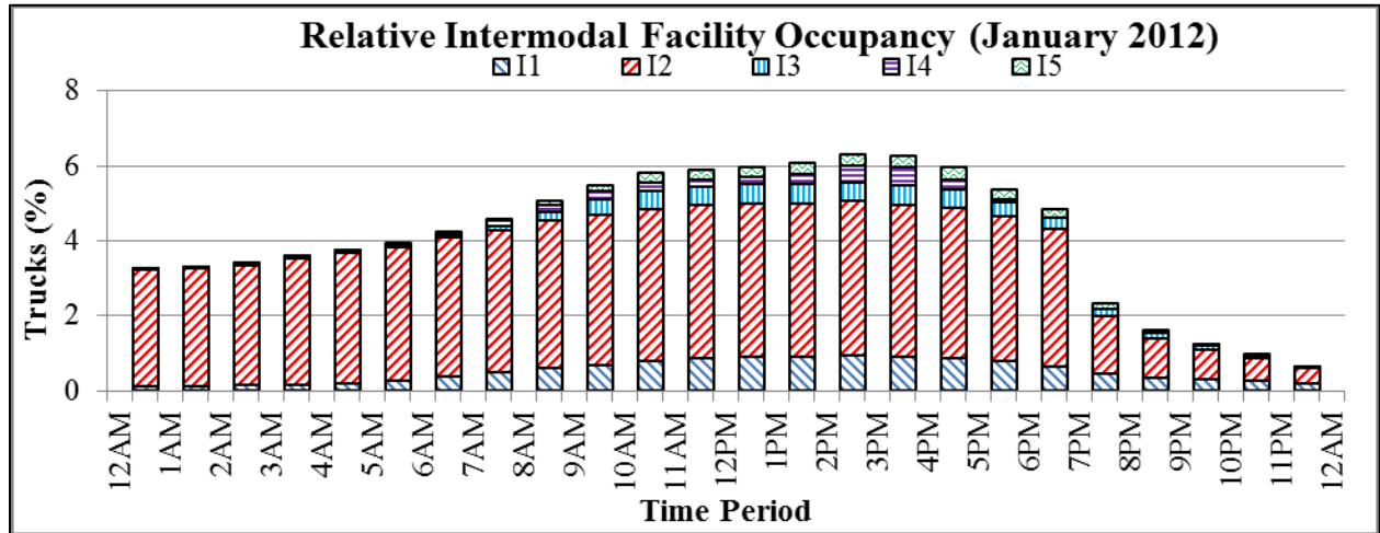
FIGURE D-1 Relative Daily Intermodal Facility Occupancy
