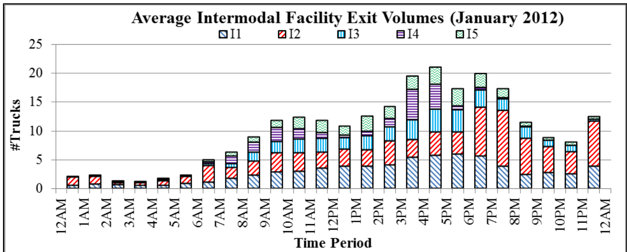
FIGURE 25 Daily Intermodal Facility Exit Volumes
