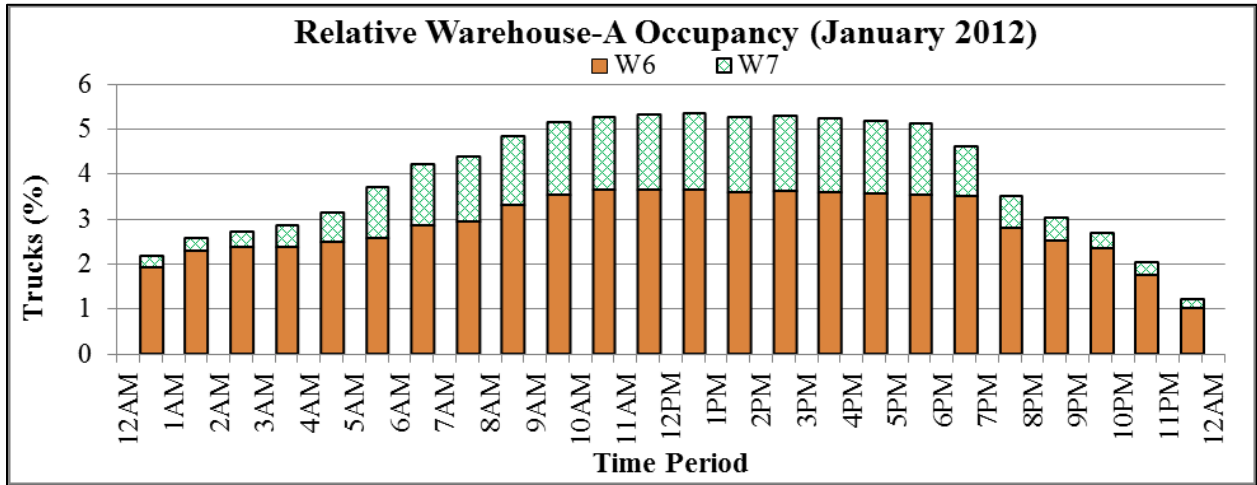
FIGURE D-7 Relative Daily Warehouse-A Occupancy
