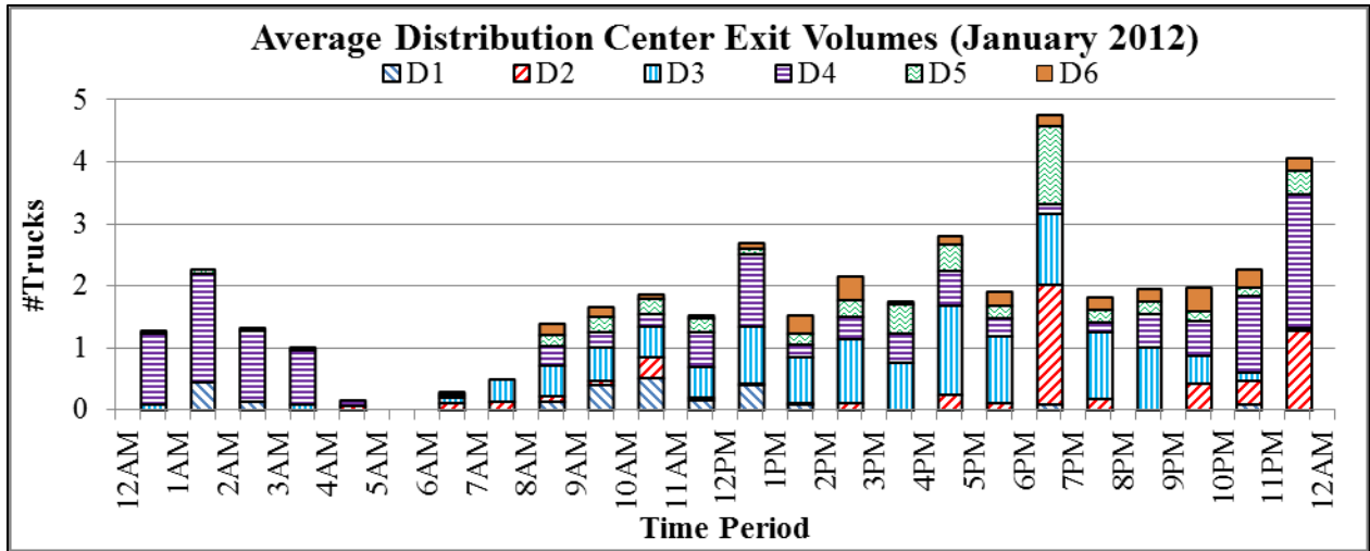
FIGURE 27 Daily Distribution Center Exit Volumes
