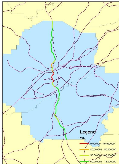
Figure 97 2014 I-65 PM Peak hour Travel Speed at Birmingham Area (TSb)
