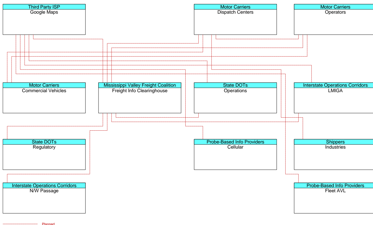
Figure 28: Interconnect Diagram
